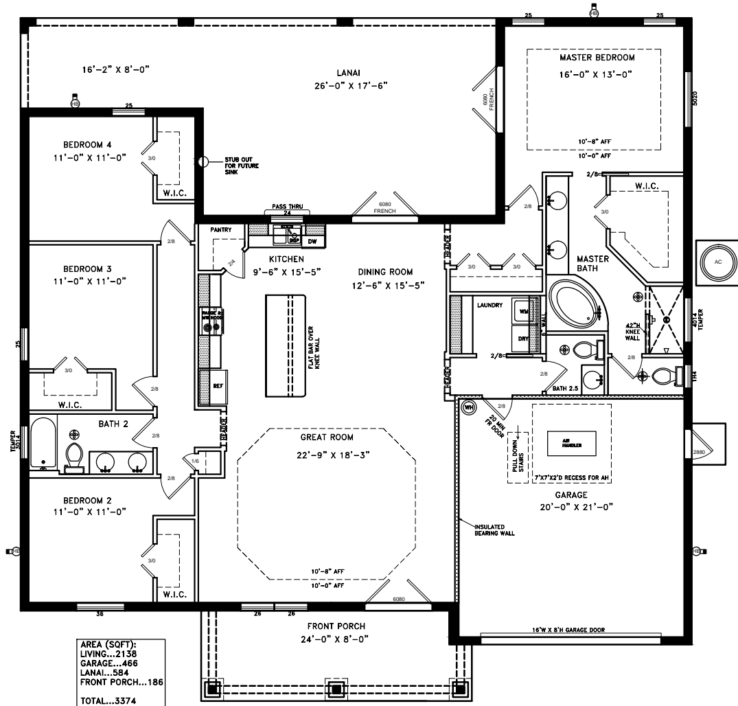
THE GAINESVILLE (59'-6"W X 60'-6"D) © COPYRIGHT TRINITY DRAFTING LLC
